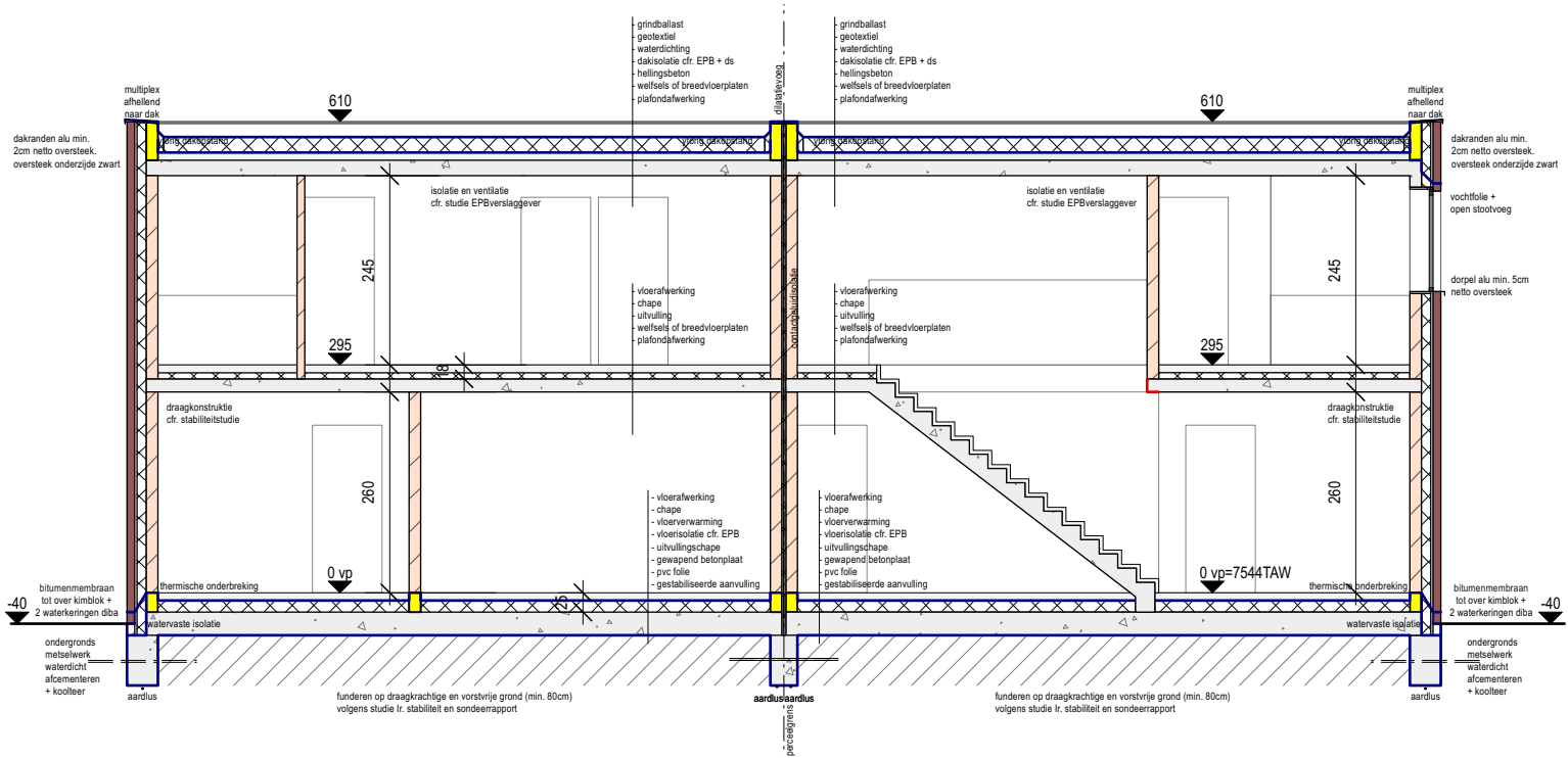
DOORSNEDE 1:100 lot 1 lot 2
